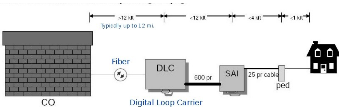
Figure 2. Telephony Feed From a DLC Cabinet
