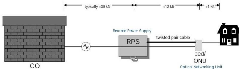
Figure 3. FTTC powered from an RPS Fiber To the Curb
