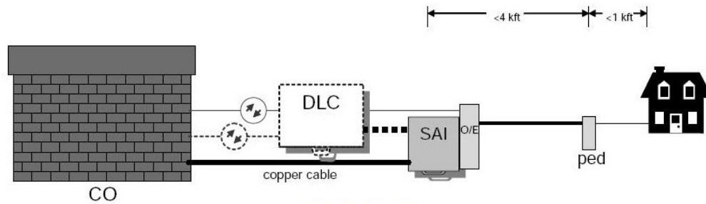
Fiber To The Node Figure 4. FTTN Architecture
